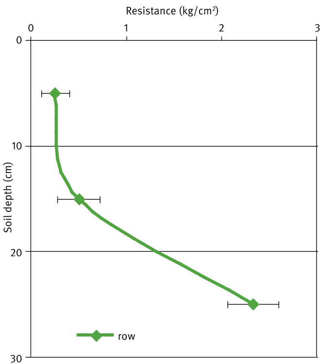
Figure 22. Soil resistance is greater in wheel tracks than row area down a soil profile to 30 cm (top graph). The shape of the resistance curve is important, a sharp increase in the resistance reading can show a subsurface compaction layer (bottom graph)
