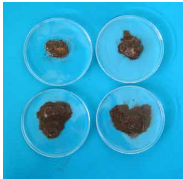
Figure 18. Low organic matter soil aggregates fall apart when wetted (bottom dishes) while those with high organic matter maintain their stability (top dishes)
