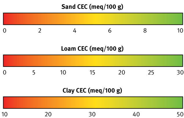
Figure 14. Guide to the interpretation of CEC values for sand, loam and clay soils
